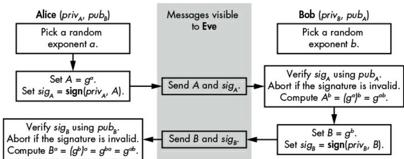
Figure 11-4: The authenticated Diffie–Hellman protocol
