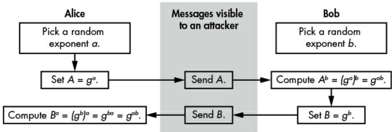
Figure 11-2: The anonymous Diffie-Hellman protocol
