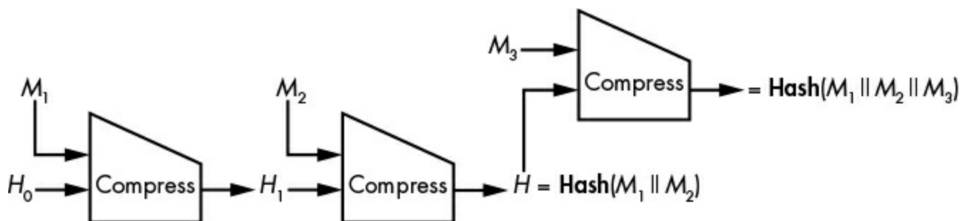
Figure 6-9: The length-extension attack
