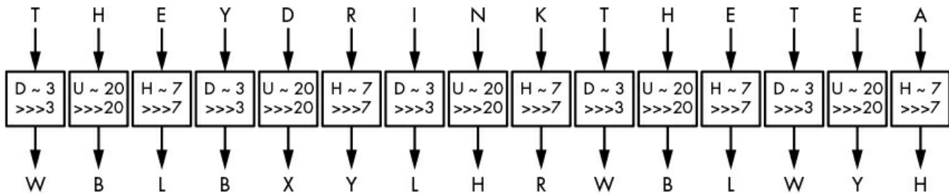
Figure 1-3: The Vigenère cipher
